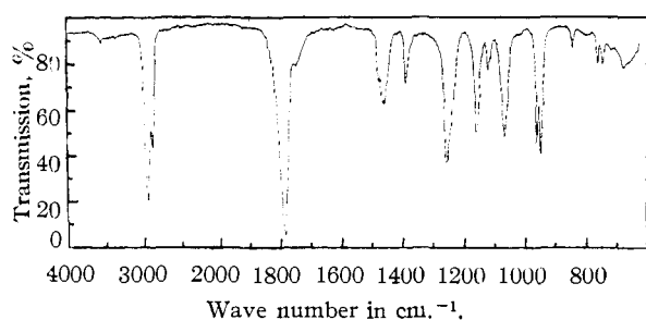
Fig. 1.—The infrared spectrum of the phosphine-pyruvic acid derivative, I (Nujol mull, Beckman IR 4 spectrophotometer).
