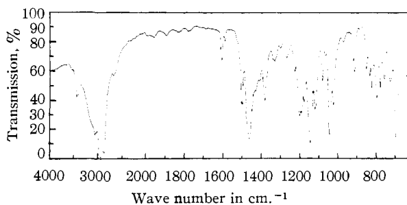
Fig. 2.—The infrared spectrum of the phosphine-benzaldehyde derivative, VII (Nujol mull, Beckman IR 4 spectrophotometer).
